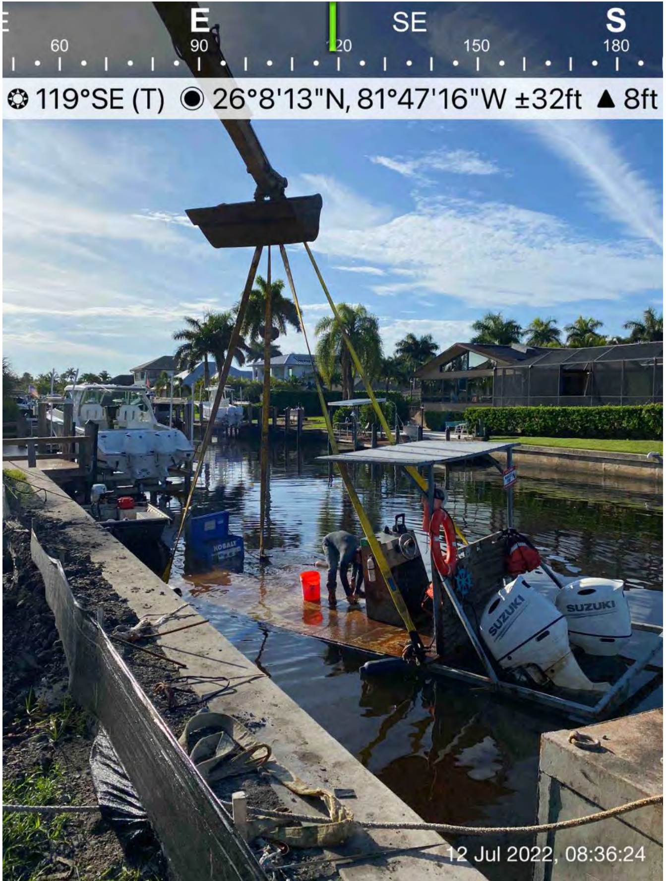
326 excavator lifting push boat and contractor opening manhole to pump water out from hull of push boat
