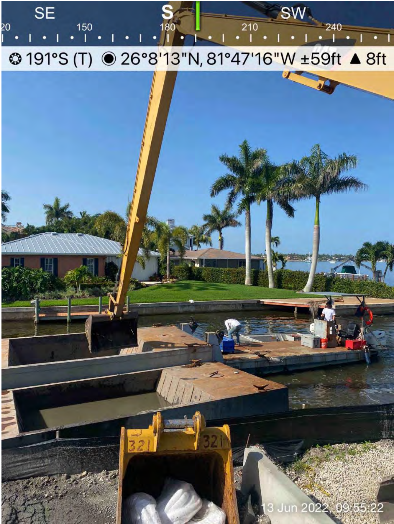
Push boat dropping off full hopper of material in Canal CC-CC
