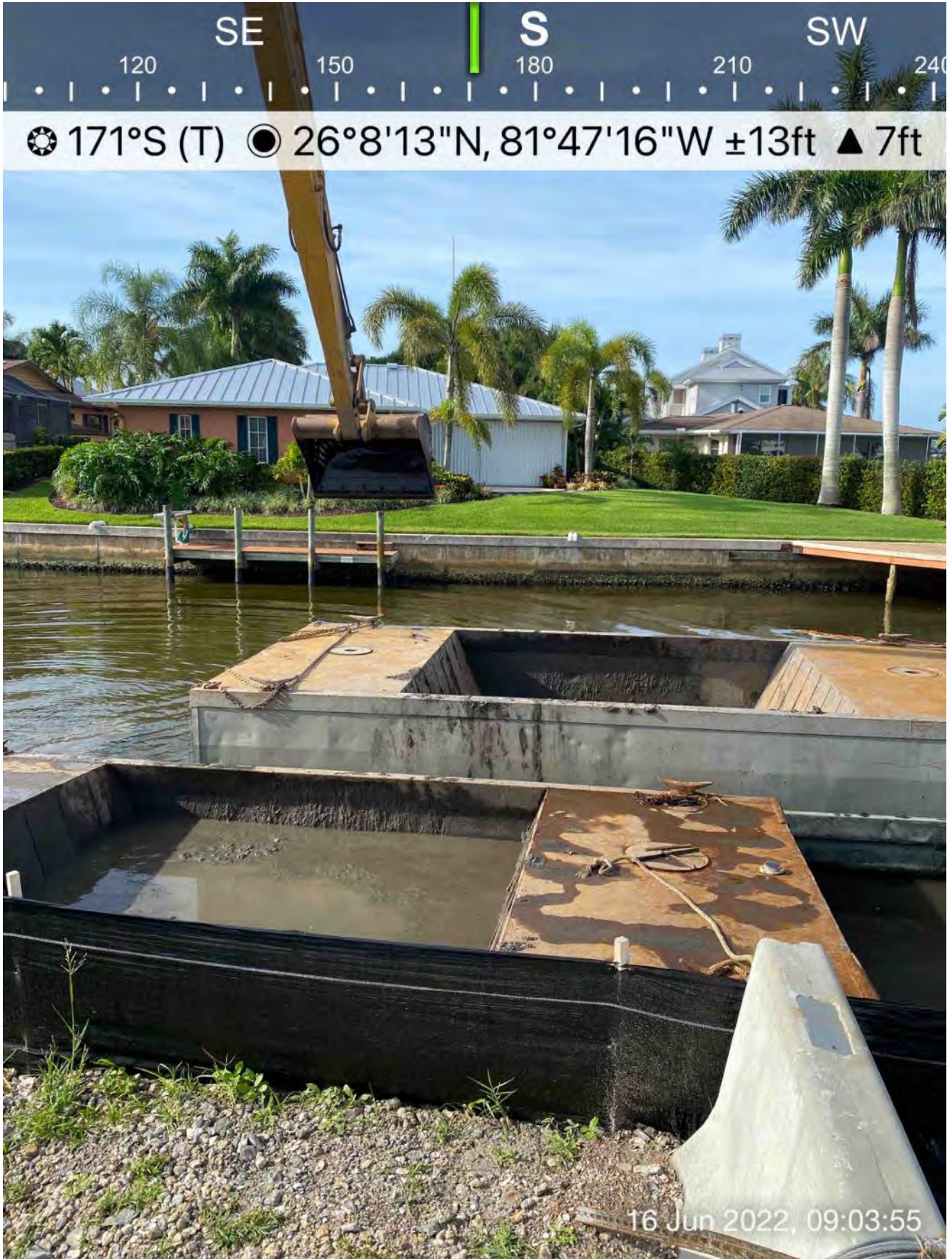
Full hopper of material and empty hopper in Canal CC-CC at station 1+50
