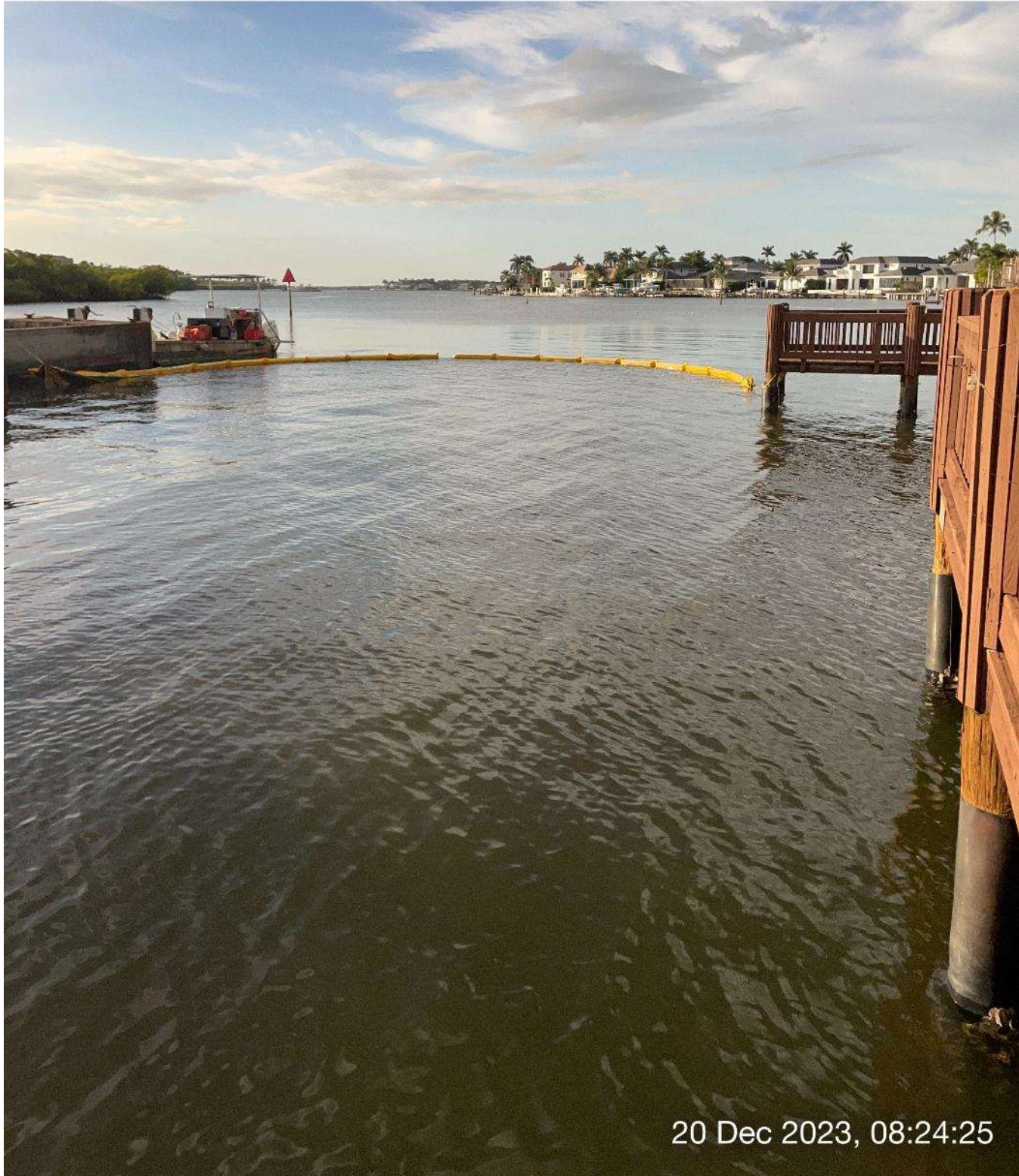
Turbidity curtain in place at station 3+00 in Canal Main B.
