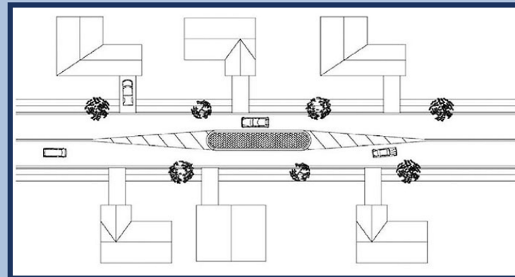
MEDIAN ISLAND
