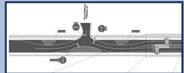
CHICANE
