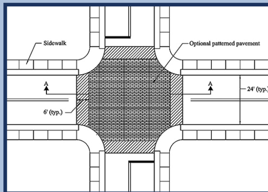
RAISED INTERSECTION
