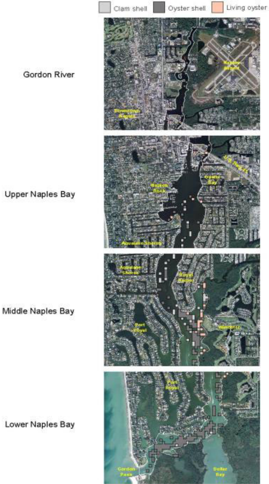
Figure 2-3. Distribution of clam shell, oyster shell and living oyster sites in the Naples Bay study area (white outline).
