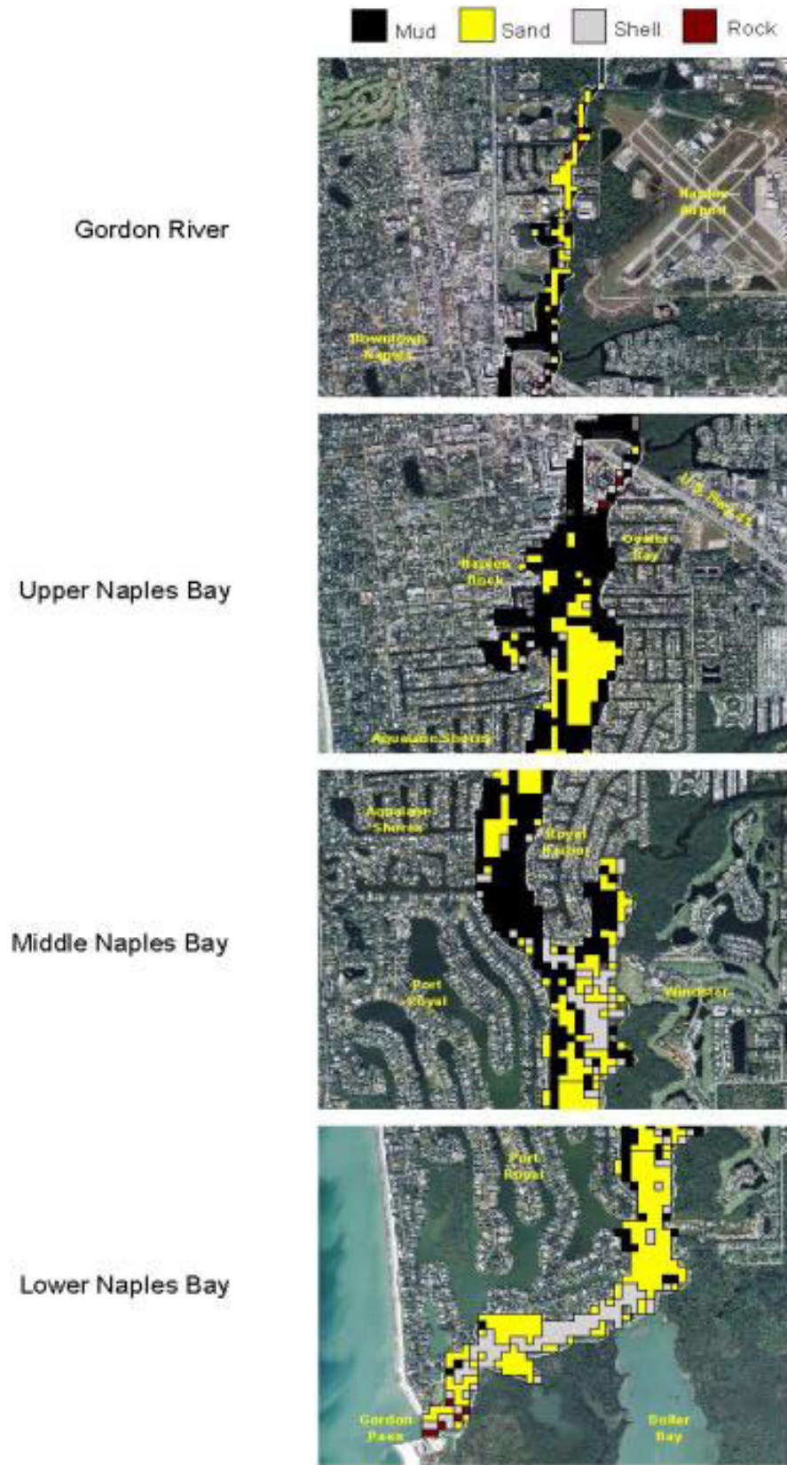
Figure 2-2. Distribution of benthic substrate sites in the Naples Bay study area (white outline).
