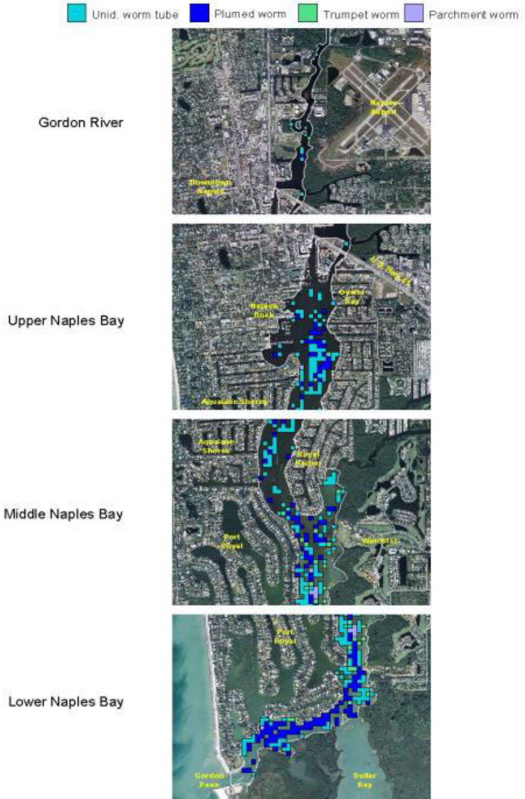
Figure 2-4. Distribution of tubicolous polychaete sites in the Naples Bay study area (white outline).
