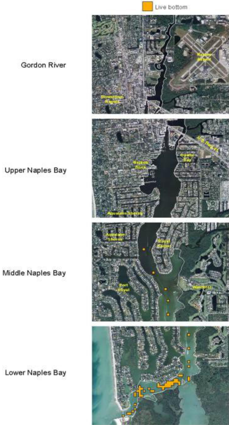
Figure 2-6. Distribution of livebottom sites in the Naples Bay study area (white outline).
