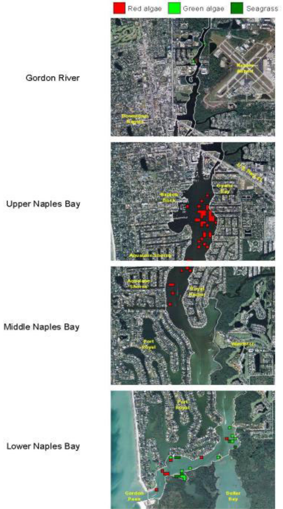
Figure 2-5. Distribution of macroalgae and seagrass sites in the Naples Bay study area (white outline).
