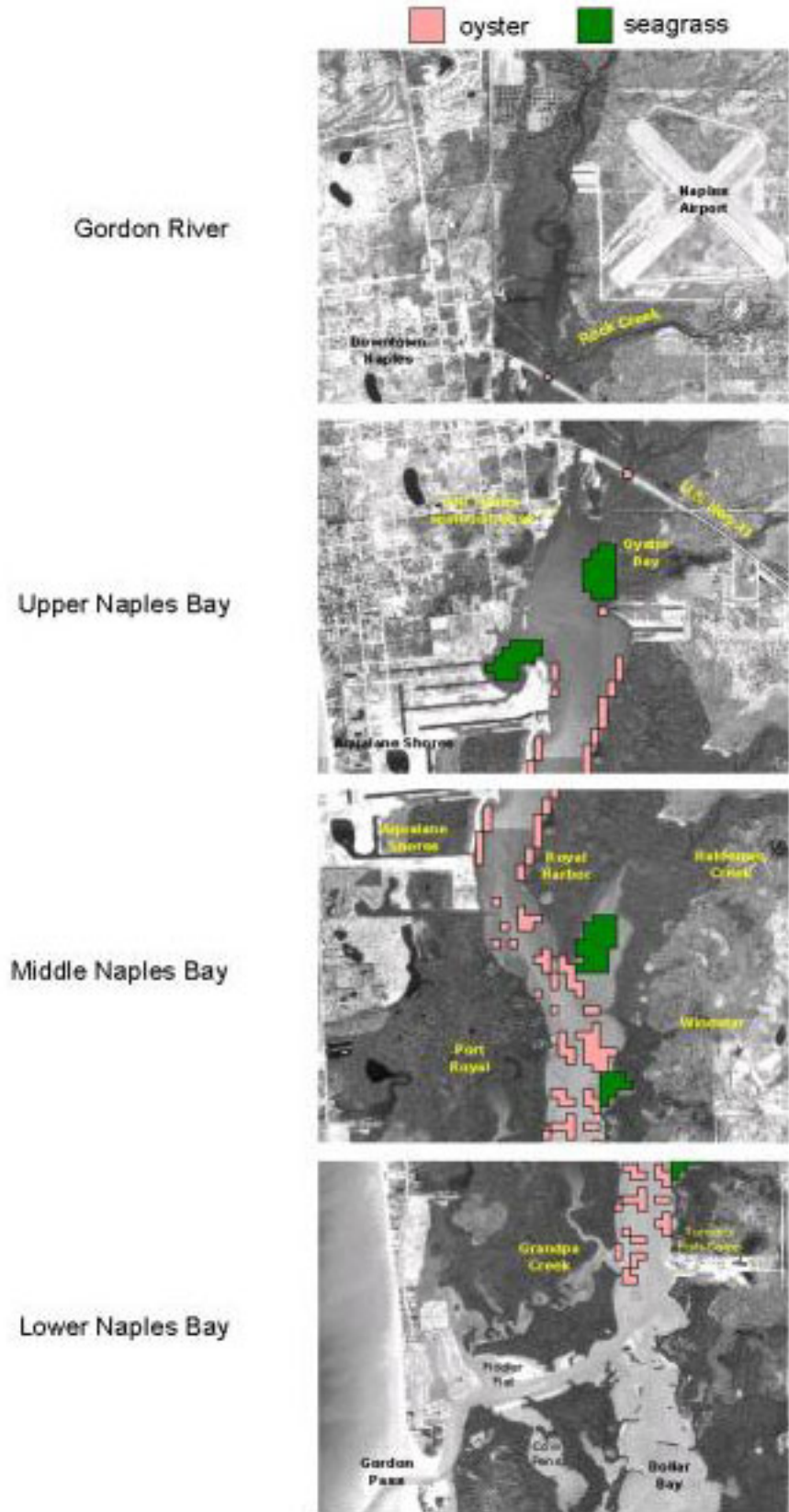
Figure 1-1. Localities in the Naples Bay area referenced in the historical narrative.
