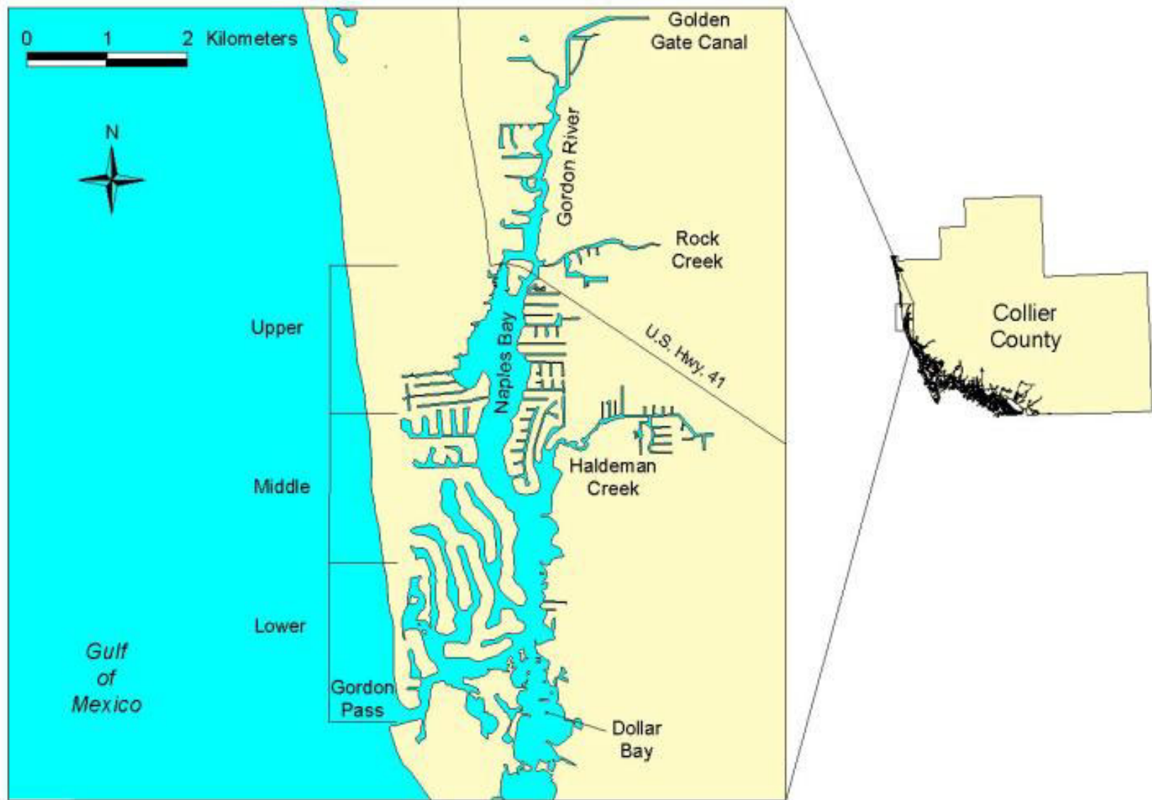
Figure 2.1. Map of west-central Collier County showing the Naples Bay study area.
