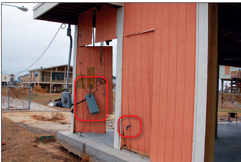
Figure 8: Utilities attached to breakaway walls that may have prevented the walls from breaking away, resulting in additional damage to the structure during Hurricane Ike in 2008 (Galveston Island, TX)
